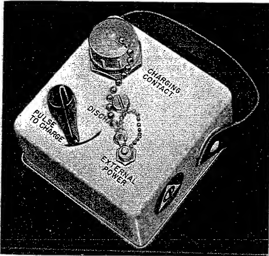
Figure 5.—Dosimeter charger.
